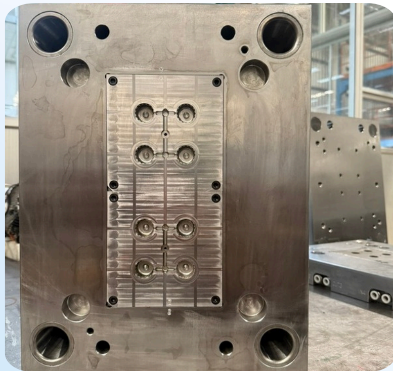
Injection Mold
